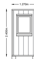
Toilet - Rear Elevation Scale - 1 : 100
