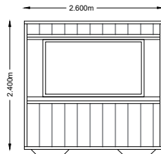
Site Welfare Facilities Container - Rear Elevation Scale - 1 : 100
