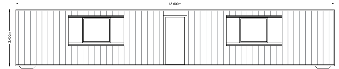
Site Welfare Facilities Container - Side Elevation Scale - 1 : 100
