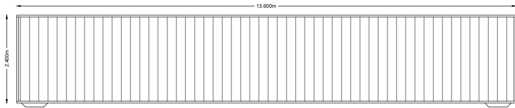
Site Welfare Facilities Container - Side Elevation Scale - 1 : 100
